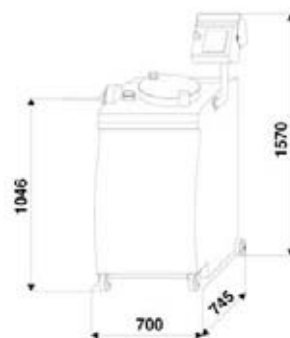
Dimensions Torsado
